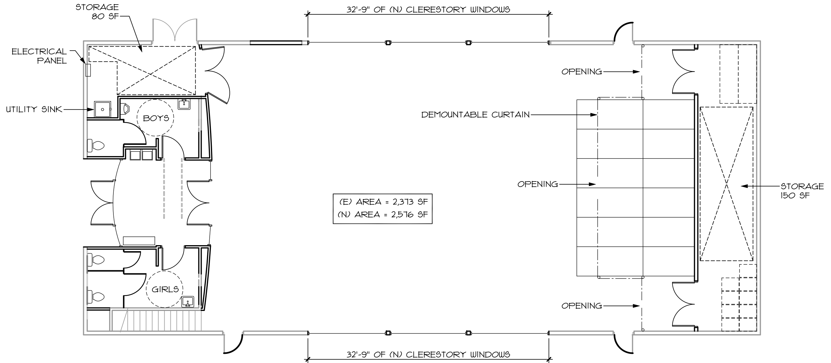
FLOOR PLAN
